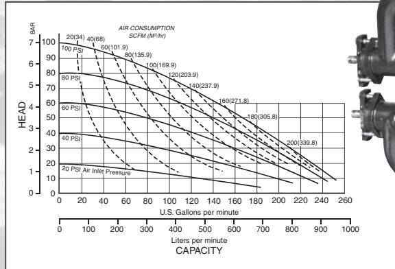
MODEL W15 Performance Curve
