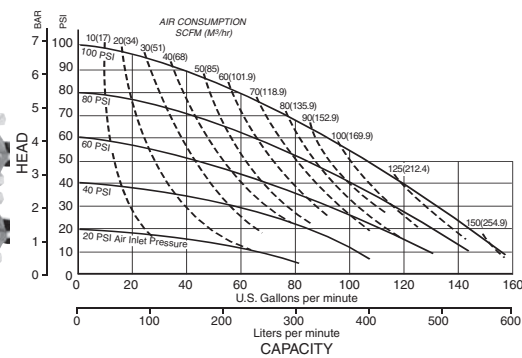
MODEL W09 Performance Curve
