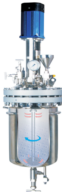
Pilot to plant scale and Gas induction reactors up to 1,000 liters
